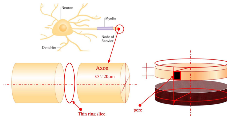
Fig. 2 N voltage-dependent ion channels on an elementary region (slice) of an axon made by a thin ring of radius \rho \approx 10 \mu\text{m} and thickness h \approx 1 \text{ nm}
