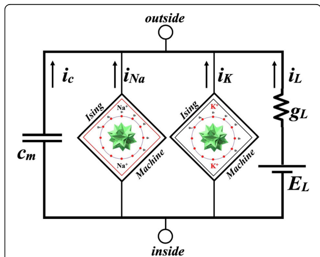
Fig. 7 The “Ising Neural Machine”. The equivalent single compartment circuit containing two stochastic elements called “Ising Neural Machines”, respectively for the Na + channels and for the K + channels [1]. By “inside” and “outside” is meant inside and outside the nerve cell membrane. The specific capacity of the membrane is indicated as c_m while i_L , g_L and E_L indicate respectively the “leakage current” [2] per unit area, the leakage conductance and potential. The currents leaving the two Ising machines are total currents (per unit area)
