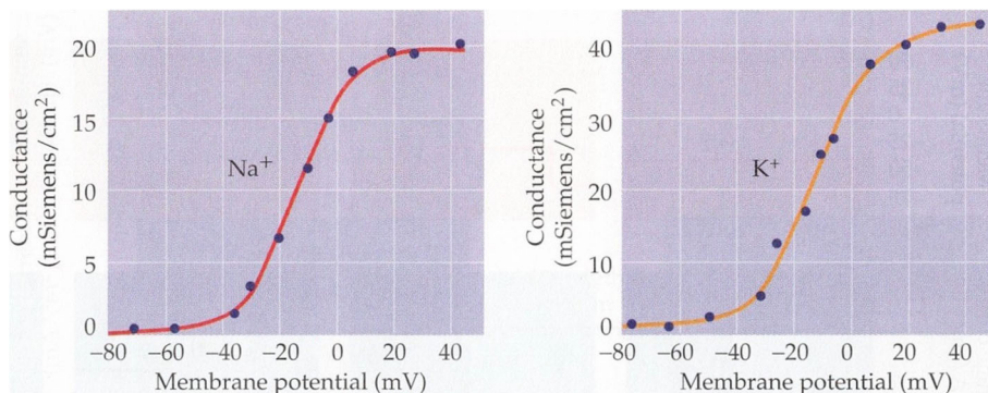
Fig. 6 Conductances as a function of the membrane potential for the Na + (left) and K + (right) channels. (Courtesy of Purves [6], after Hodgkin and Huxley [2])
