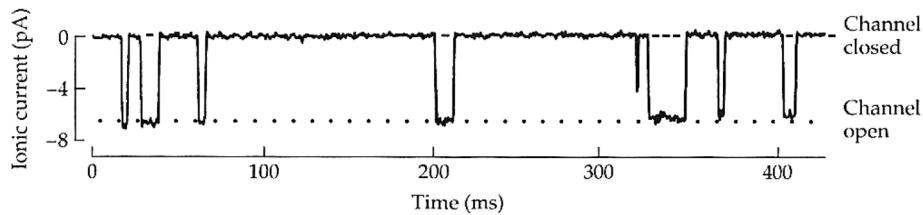
Fig. 1 The flow of an ionic current of the order of 6.6 pA through a small axonal membrane element shows eight ion channel openings (corresponding to a flow of 4.1 \times 10^7 ions per second through a single pore). (Courtesy of B. Hille, [5])
