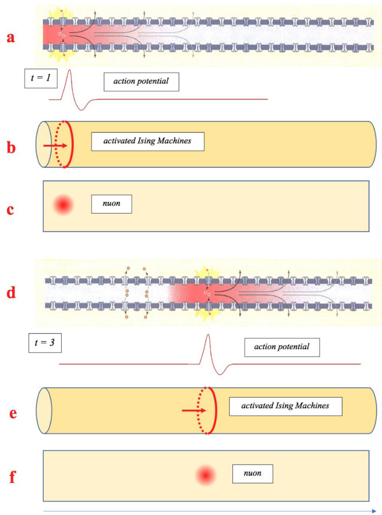
Fig. 9 Spikes and nuons. a and d (modified after D. Purves, [6]), show the motion of a spike for t = 1 and t = 3 (arbitrary units). b and e show the trigger of a pair of \text{Na}^+/\text{K}^+ Ising machines housed in annular regions of the membrane for t = 1 and t = 3 (arbitrary units). c and f show the motion of a nuon along the axon for t = 1 and t = 3 (arbitrary units)
