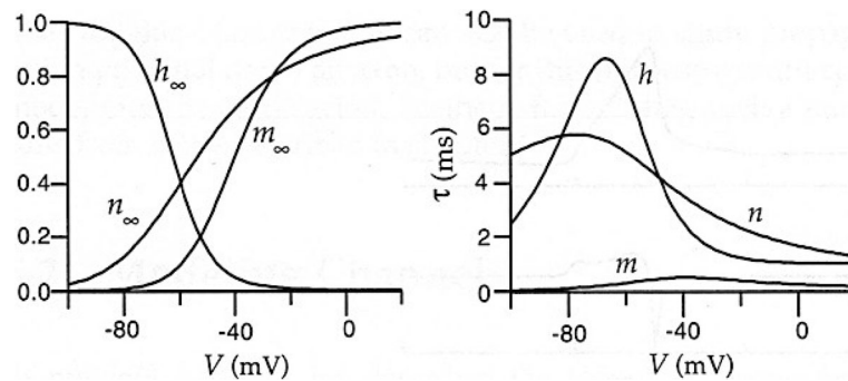
Fig. 5 Characteristic limit ratios as a function of membrane potential in the HH model. The figure on the left shows the limit functions for activating the K^+ conductance ( n_\infty ) and the activation and inactivation functions for the Na^+ conductance ( m_\infty, h_\infty ). The relative time constants (as a function of potential) are shown on the right. (courtesy of P. Dayan et Al., [8])
